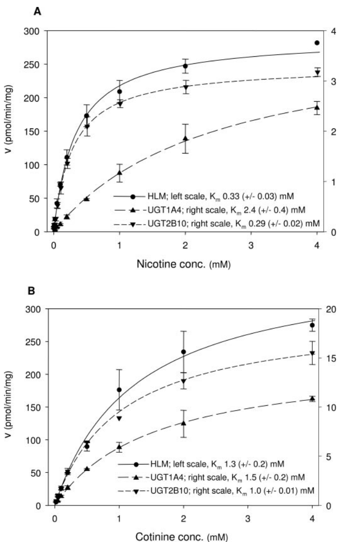
Fig. 5. Kinetic analyses of the glucuronidation of nicotine (A) and cotinine (B) by HLMs and recombinant human UGT1A4 and UGT2B10. The glucuronidation rates, v , for the HLMs are presented on the left-hand side of the y-axis, whereas the right-hand side values are for the non-normalized rates of the recombinant UGT samples. The rates represent the mean ( \pm S.D.) of two to four independent determinations. The calculated K_m ( \pm S.E.) values for the substrate, derived from the Michaelis-Menten equation, are also presented (see Materials and Methods for further technical details).
