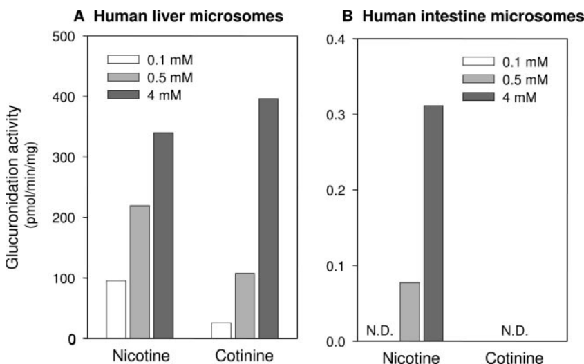
Fig. 7. Activity analyses of human microsomes from either the liver (A) or intestine (B; the microsomes were from the duodenum and jejunum sections of the intestine) in N -glucuronidation of nicotine and cotinine. Three different substrate concentrations were used in the assays. Note the differences in y-axis units between A and B. Activities were determined in duplicate (<10% difference). N.D., no detectable activity or activity below quantification limit (0.04 and 0.08 pmol/min/mg for nicotine and cotinine, respectively).
